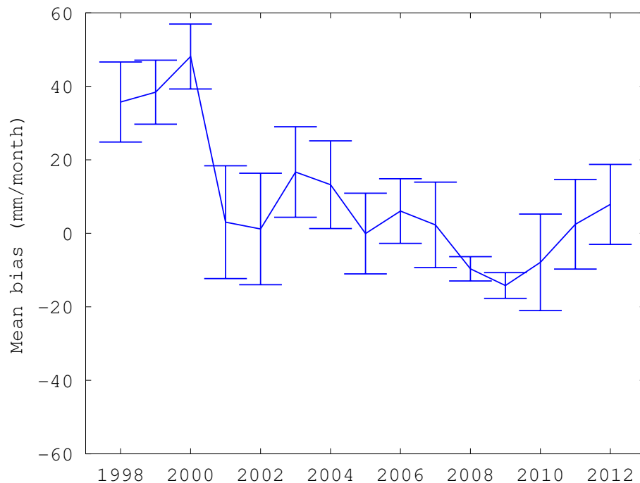
Figure 3. Mean bias in the TRMM precipitation product, compared to Nepal station observations, by year. Error bars show the standard error of the bias over each year.
